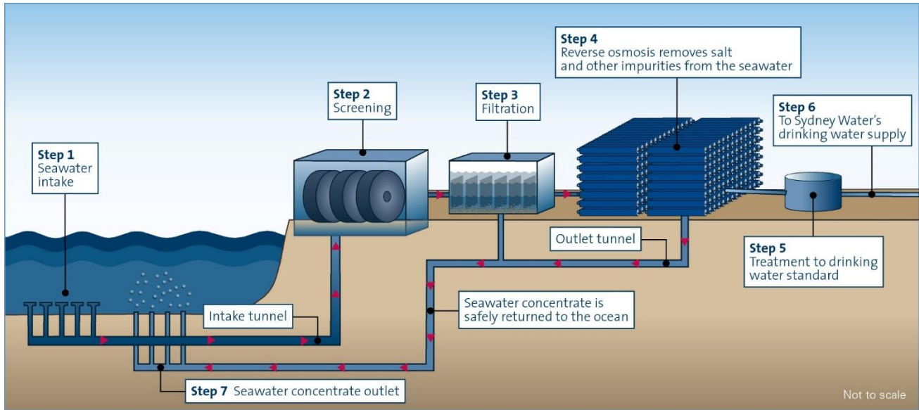
Fig. 7: Reverse Osmosis desalination process schematic [11].
