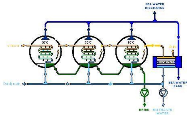
Fig. 4: Multiple-effect distillation schematic[8]
