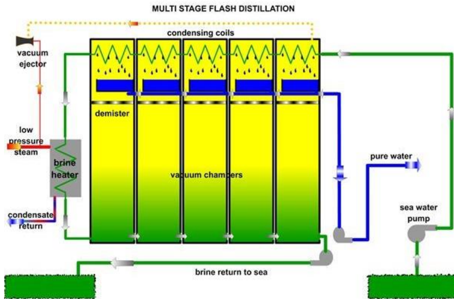
Fig. 2: Multi-stage flash distillation schematic [5]
