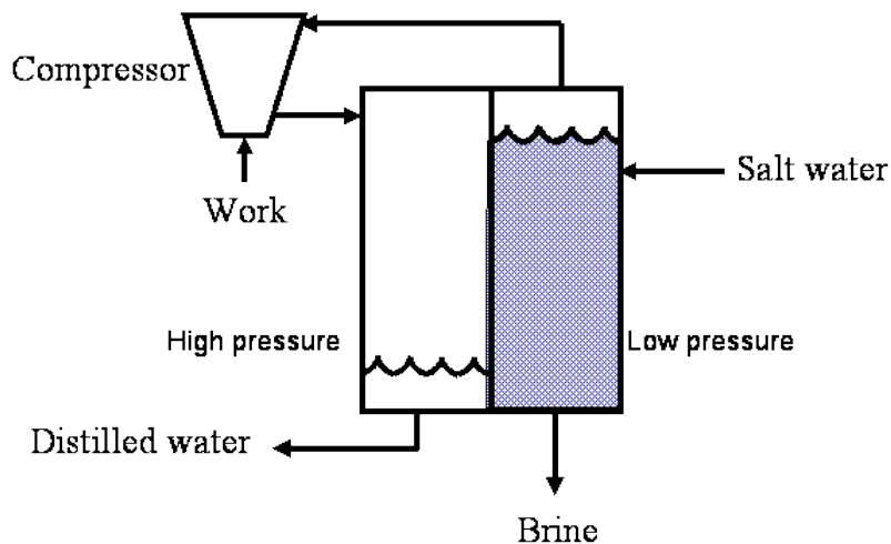
Fig. 6: Vapor compression process schematic.
