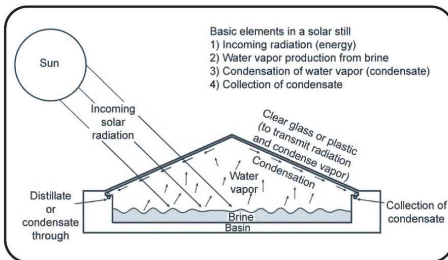
Fig. 12: Sustainable Desalination System[14].
