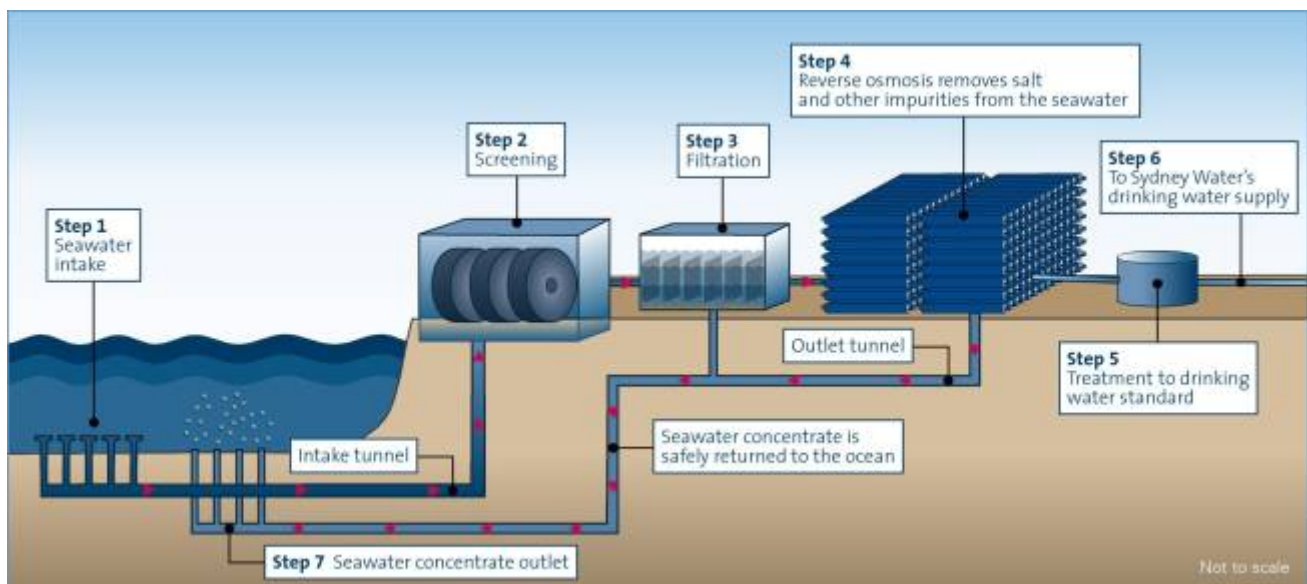
Figure 8: Reverse osmosis desalination process schematic [10]
