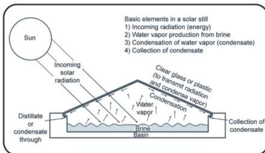
Figure 11: Solar desalination schematic [13]
