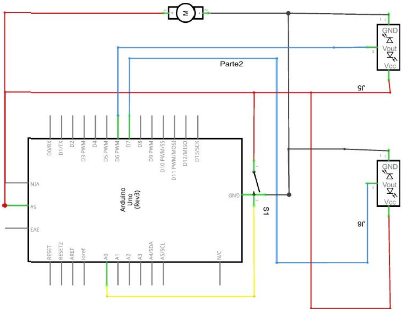
Figure 53: Arduino schematic
