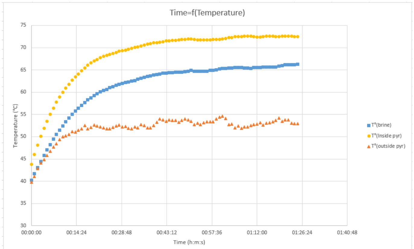
Figure 49: Time=f(Temperature)
