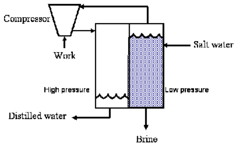
Figure 5: Vapor compression process schematic [7]
