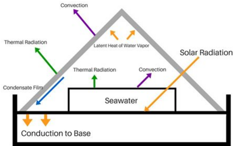
Figure 48: Thermodynamic scheme
