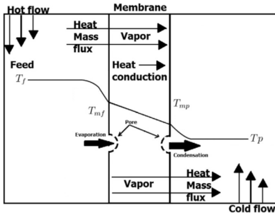
Figure 9: Direct Contact Membrane Distillation schematic [11]
