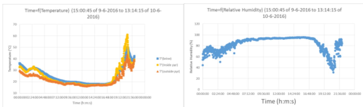
Figure 51: Temperature (A) and Relative Humidity (B) of the system during a 24 h test
